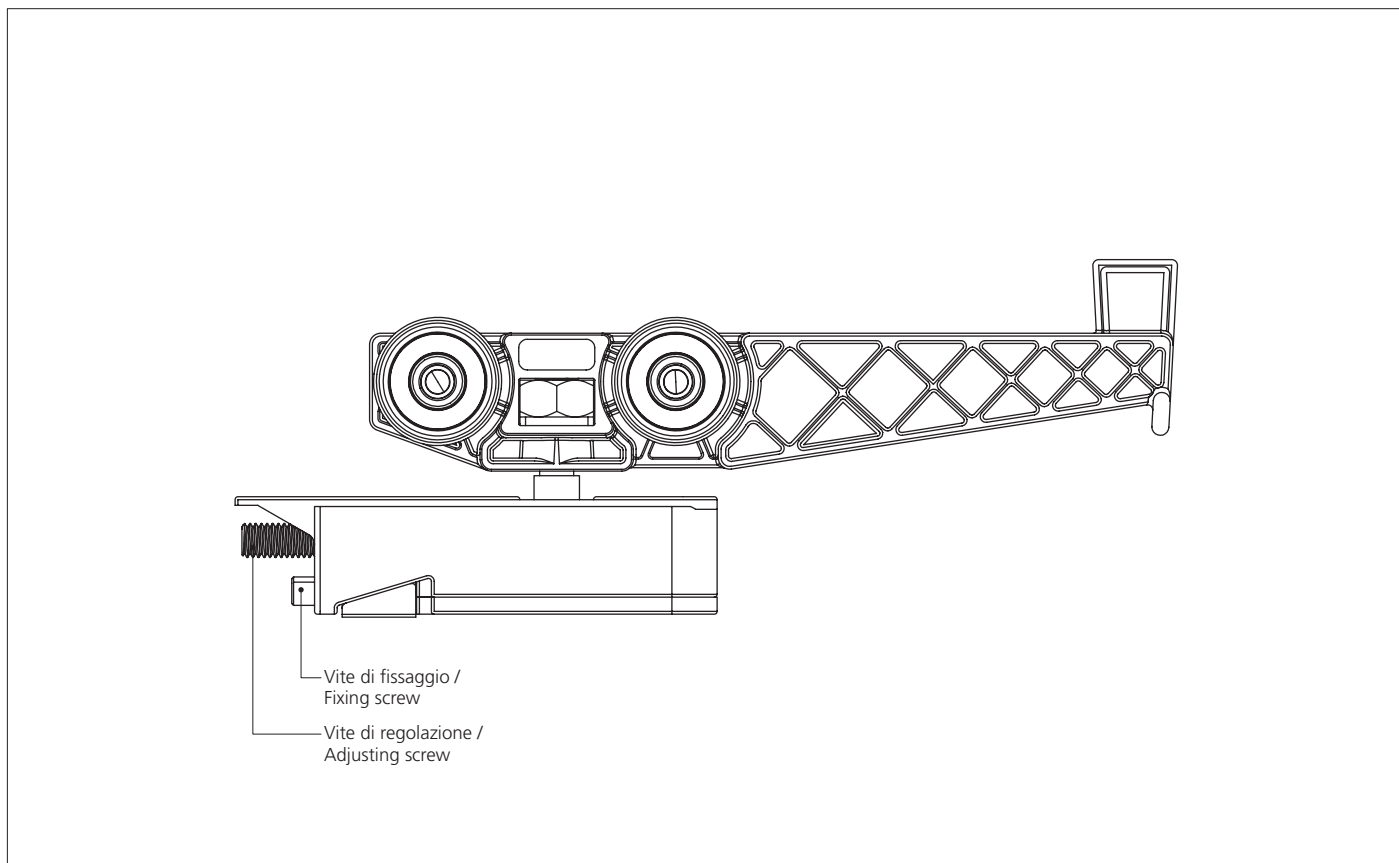
Carrello. Carriage.
