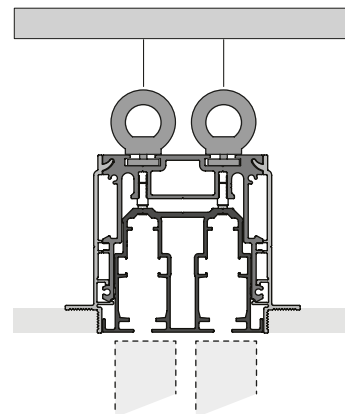
versione appendinata (A) hanging version (A)
