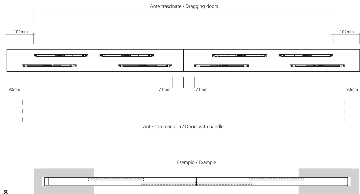
Vista in planimetria / Plan view
